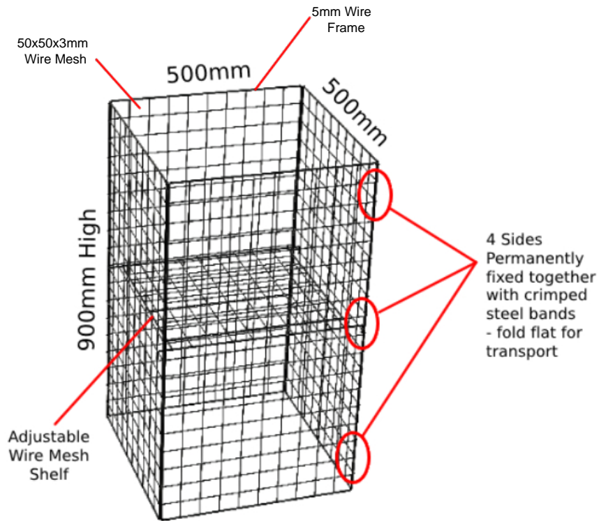
Collapsible Square Dump Bin
