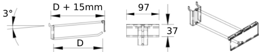
Single Pegboard Hook with Plastic PI Flipper
