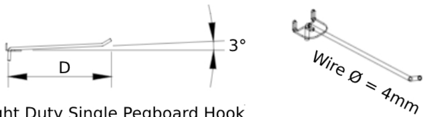
Light Duty Single Pegboard Hook
