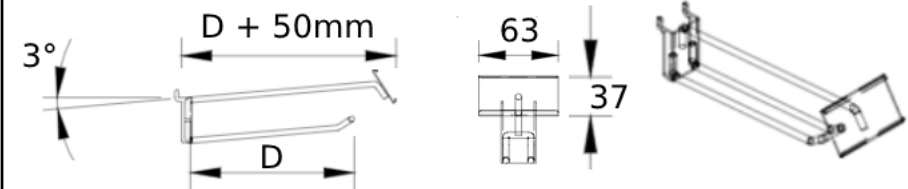
Double Pegboard Hook with 63mm Slide In PI Label
