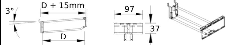
Double Pegboard Hook with Plastic PI Flipper
