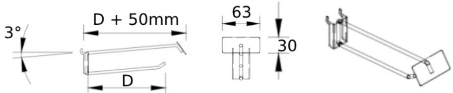
Single Pegboard Hook with Flat PI Label
