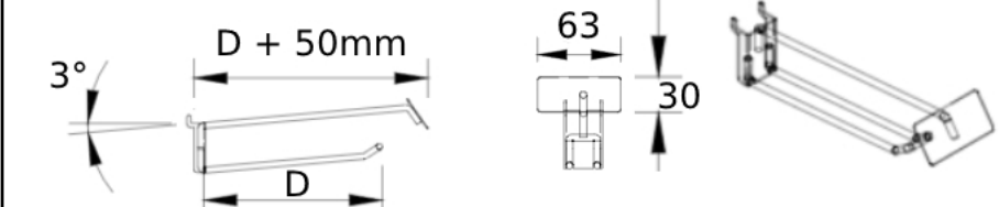
Double Pegboard Hook with Flat PI Label
