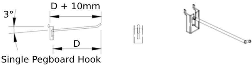
Light Duty Single Pegboard Hook
